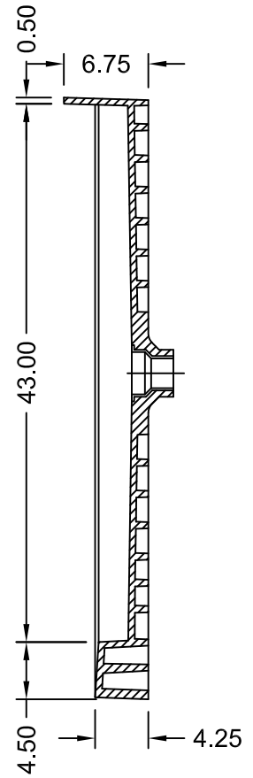
SECTION B-B
